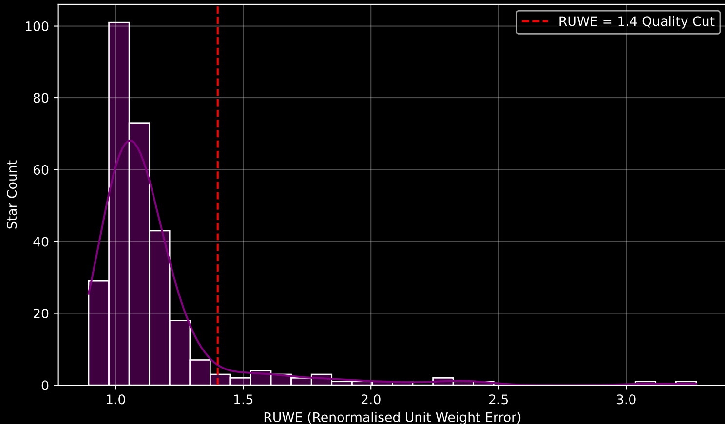
GAPOGEE DR17 Field [169+18_btx] RUWE Distribution (n= 298)
