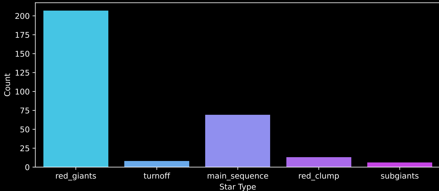
APOGEE DR17 Field: [169+18_btx] Count plot of Star Type
