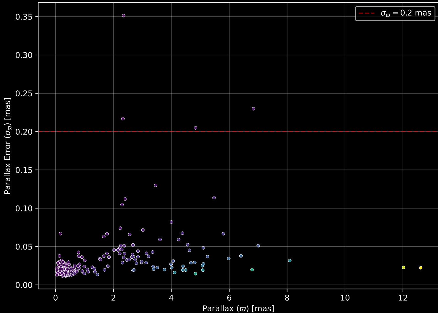
APOGEE DR17 Field: [169+18_btx] Parallax Quality (n= 303)
