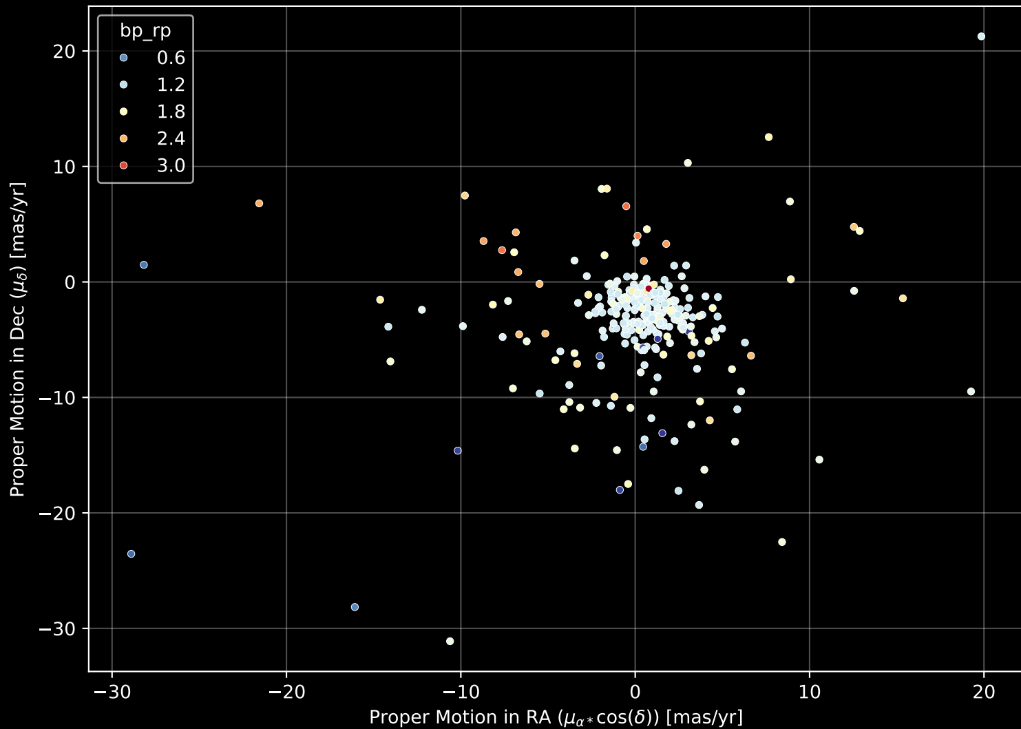
APOGEE DR17 Field: [169+18_btx] Proper Motion Diagram (n= 303)
