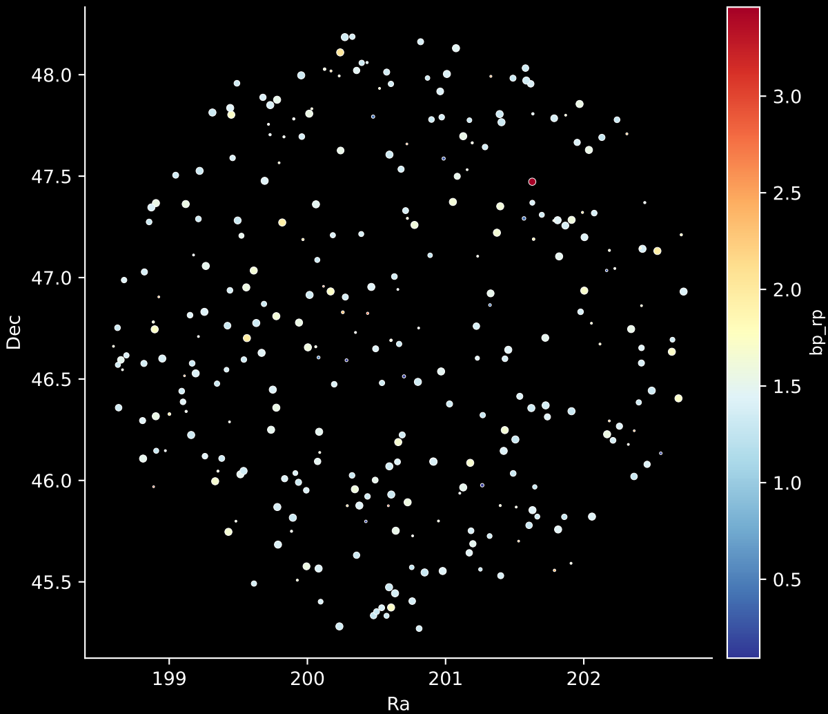
APOGEE DR17 Field: [169+18_btx] Stars: 303
