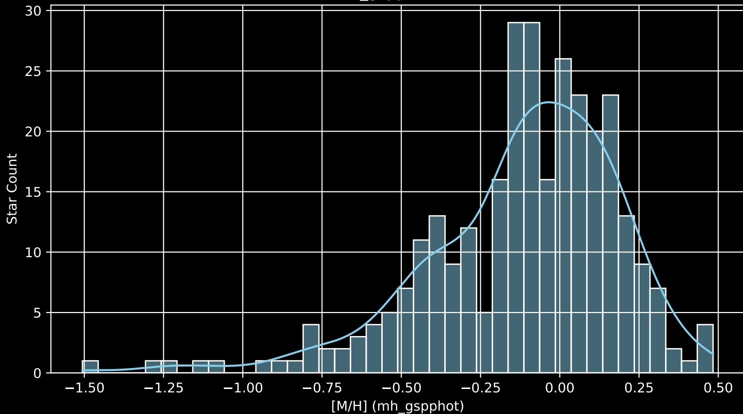
APOGEE DR17 Field: [169+18_btx [M/H] (mh_gspphot) (n= 303)
