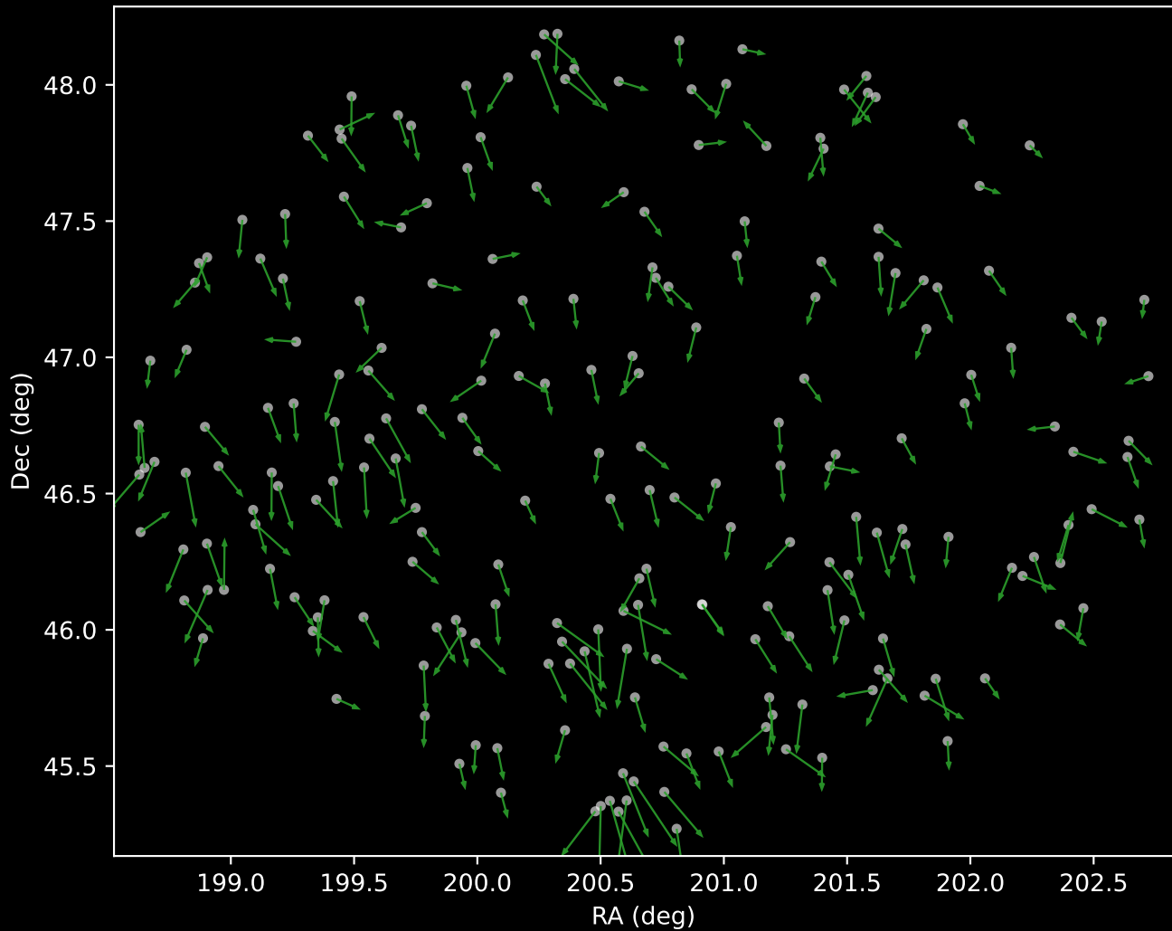
APOGEE DR17 Cluster 4 Proper Motion Vectors (n=218)
